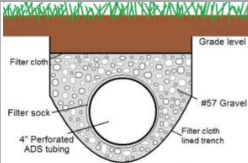
French Drain
