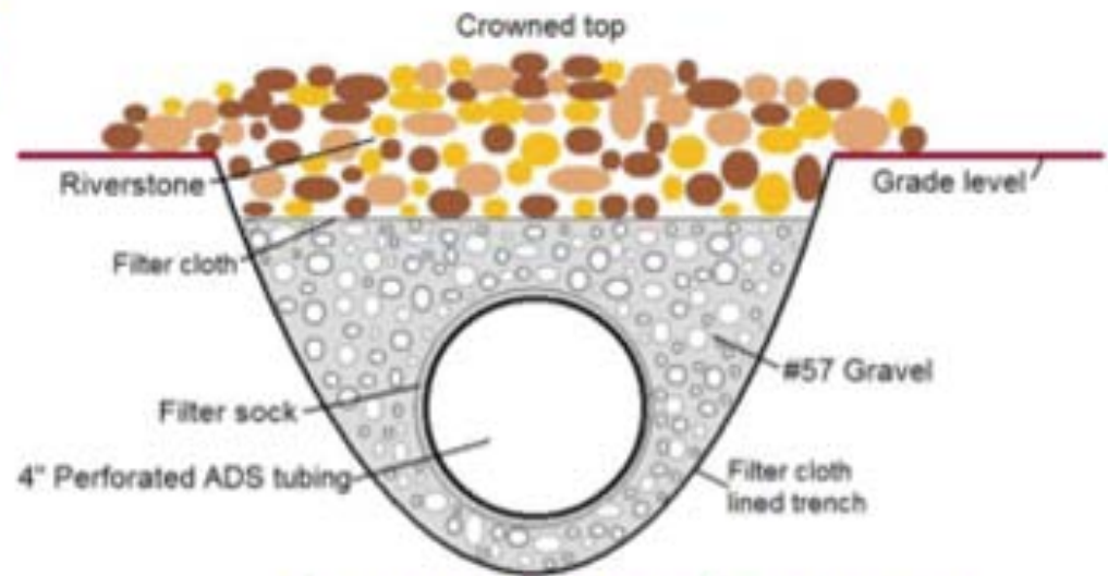
Open French Drain
