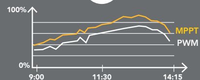
CHARGING EFFICIENCY VS TIME
