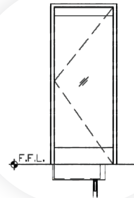
SECTION 4440-S
