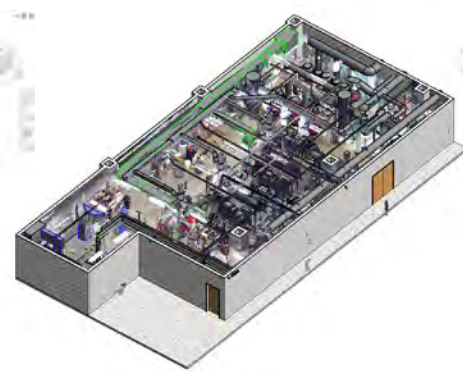
DATA-ACCURATE BUILDING INFORMATION MODEL
