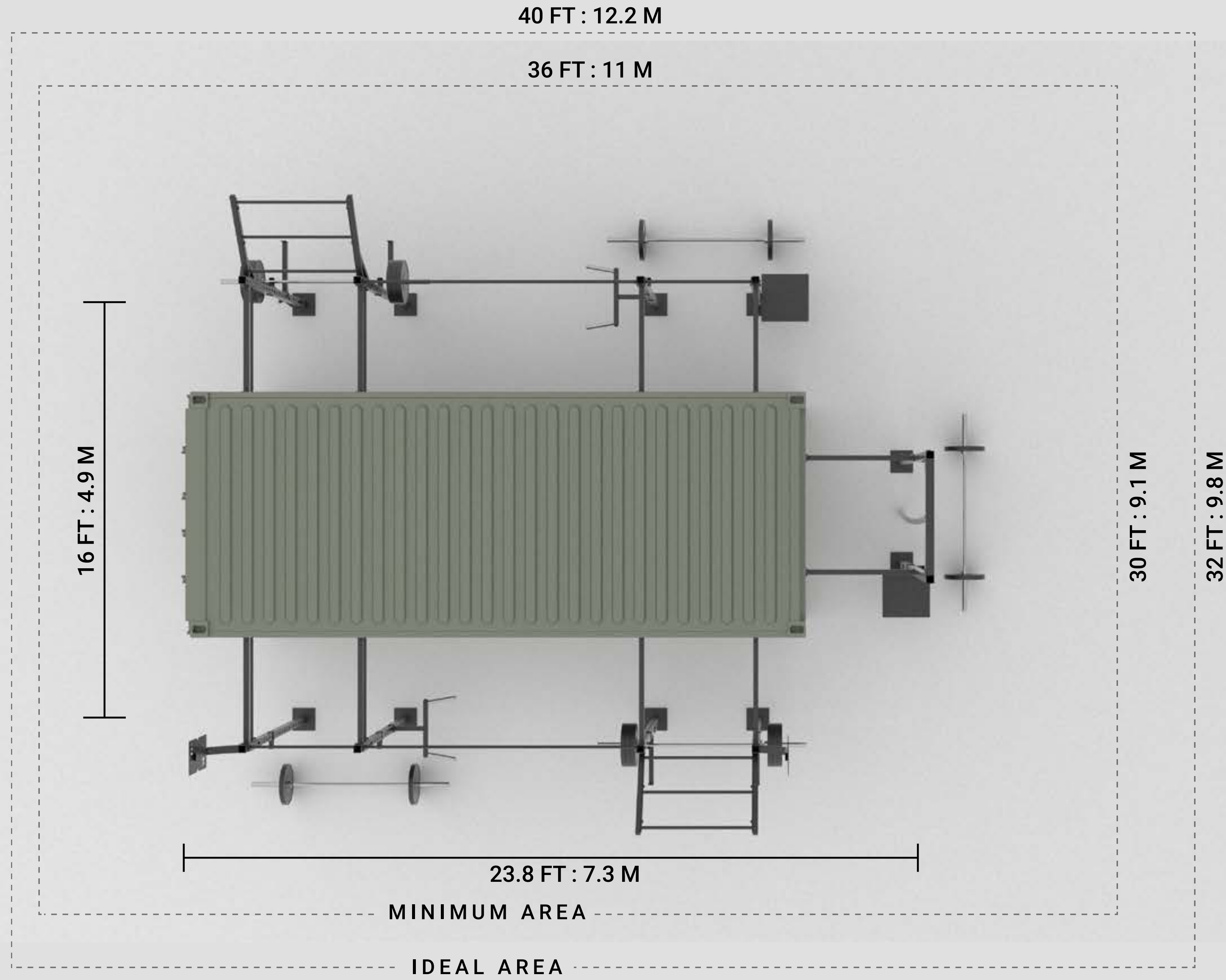
20FT LOCKER DIMENSIONS
