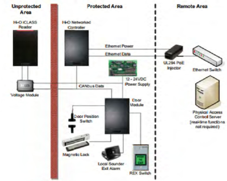
FIGURE 1 - NETWORK CONTROLLER
