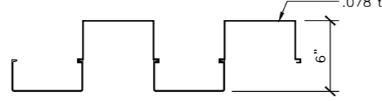
4" x 6" SELF-MATING DECK
