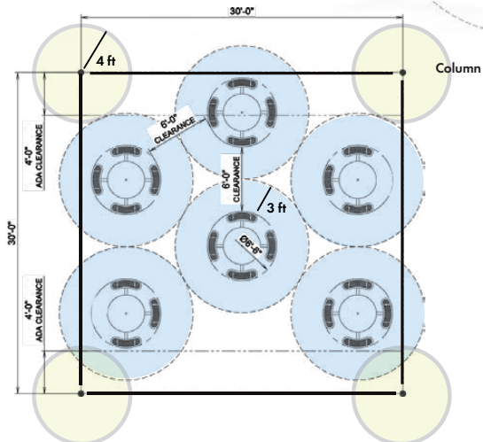
30'x30' Structure - Seats up to 24 (Minimum of 2 ADA Accessible seating areas)
