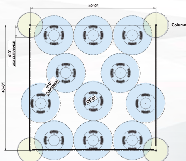
40'x40' Structure - Seats up to 44 (Minimum of 3 ADA Accessible seating areas)
