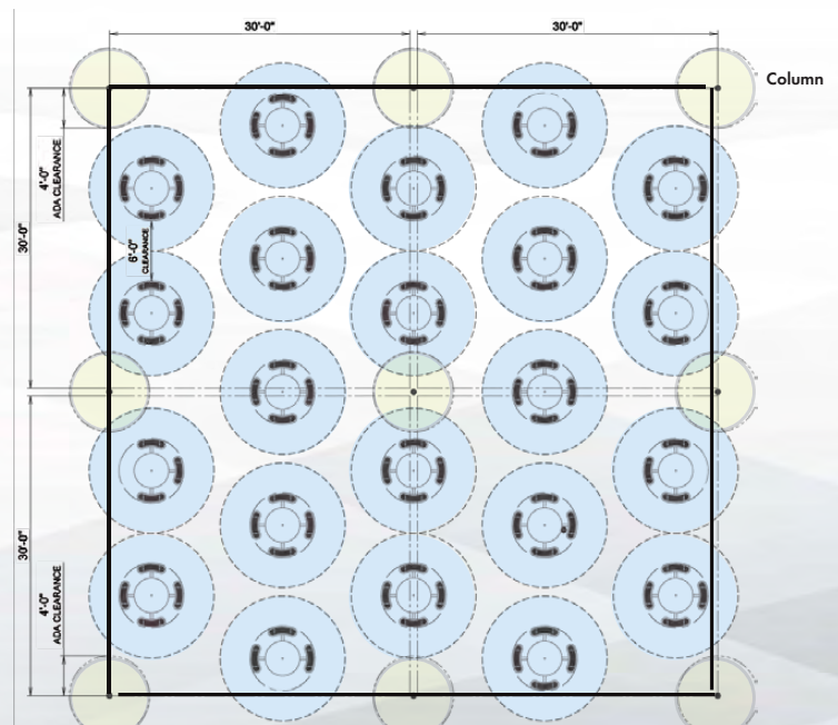
60'x60' Structure - Seats up to 88 (Minimum of 5 ADA Accessible seating areas)
