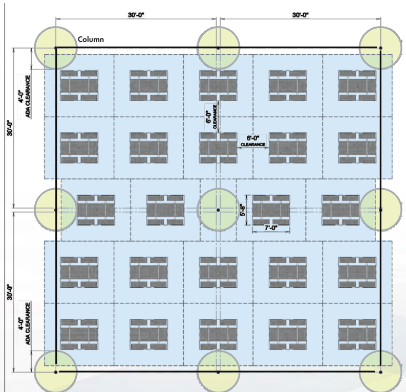
60'x60' Structure - Seats up to 96 (Maximum of 48 ADA Accessible seating areas)
