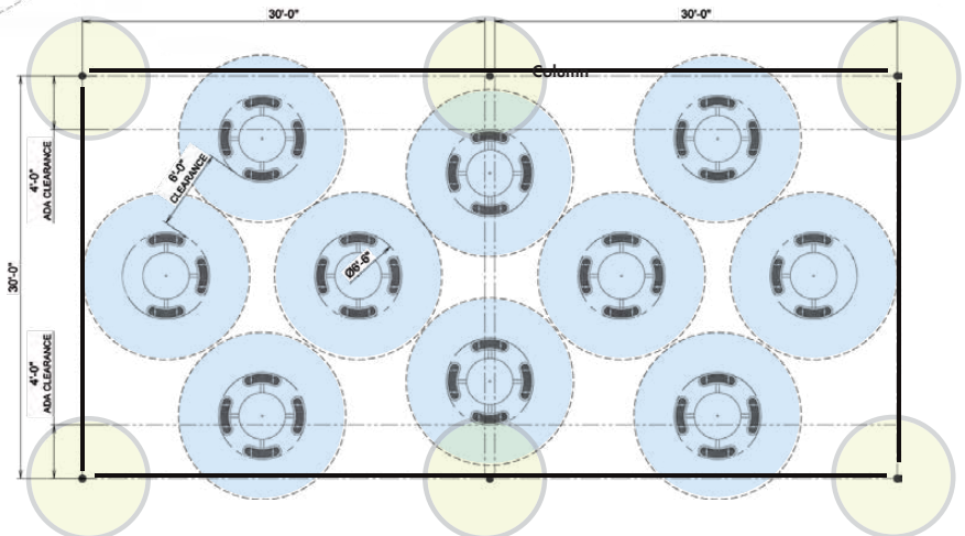
30'x60' Structure - Seats up to 40 (Minimum of 2 ADA Accessible seating areas)
