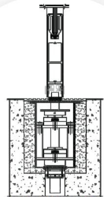
SECTION 4440-S
