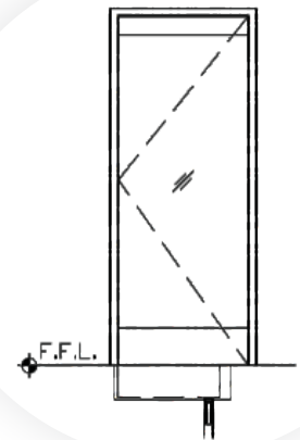
SECTION 4440-S
